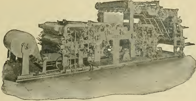
FIRST PERFECTING PRESS.
